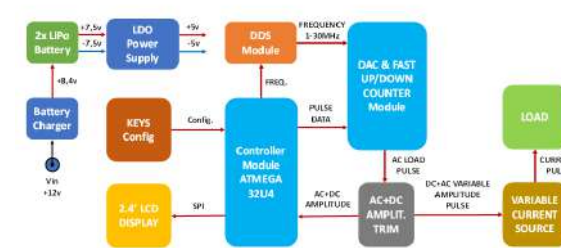
Load Dump Device, Block Diagram
